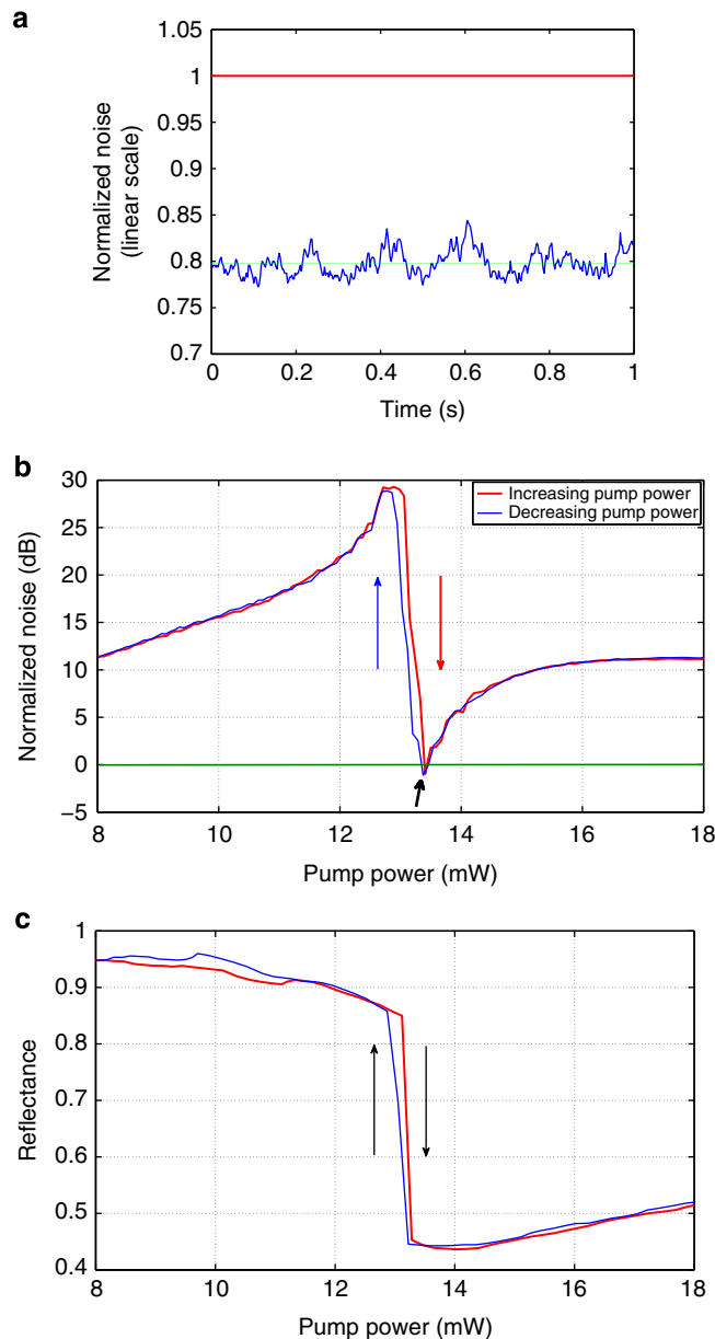
Figure 3 | Intensity squeezing and bistability. (a) Squeezed intensity noise at fixed pump power near the lower turning point (linear scale), on a 6 \mu\text{m} pillar at cavity-exciton detuning of -5 meV and a polariton-laser detuning of 0.19 meV. The noise data were normalized with a measurement of the shot noise and a measurement of the dark noise, with S(t) = (\text{noise}(t) - \langle \text{dark}(t) \rangle) / (\langle \text{shotnoise}(t) \rangle - \langle \text{dark}(t) \rangle) , \langle \dots \rangle being the time average. The measured noise reduction is 20.3 \pm 1.5\% ( -1 dB) below the shot noise limit before corrections, 35.8 \pm 2.6\% after. The dashed green line is the average noise and the red line is the shot noise. (b) Intensity noise (spectral noise power, semi-logarithmic scale) as a function of the pump power for the same pillar under the same conditions as in a. The noise increases smoothly towards a peak just before the bistability threshold, then suddenly drops to form a gap where intensity squeezing is observed, with about the same value as in a. Here also the normalized spectral noise is obtained with three measurements (noise, shot noise and dark noise). In red is the curve obtained by increasing the pump power, in blue is the curve obtained by decreasing the pump power and the green line represents the shot noise (normalized to one). The thick black arrow points to where a was recorded. (c) Bistability curve obtained by plotting the reflectance versus the pump power, for the same pillar under the same conditions as in a,b. The colour code is the same as in b. Above the thresholds the transmission is increased, hence a sharp reduction on the reflectance.
